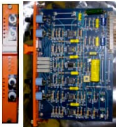
PID Board Front View Side View
